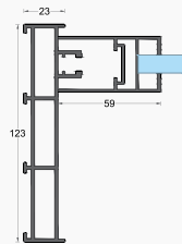
3 TRACK SIDE FRAME
