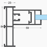
2 TRACK SIDE FRAME
